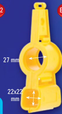
Nipple Pipe Hanger With Clamp
